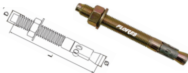
Conexpand metallic fara camasa
