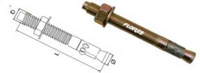
Conexpand metallic fara camasa
