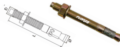
Conexpand metallic fara camasa
