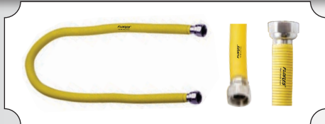
Racord gaz metalic izolat (Piulita+Piulita) de 3/4
